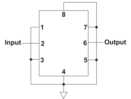
Single-ended Input and Output Filter Alternate Connection Diagram
