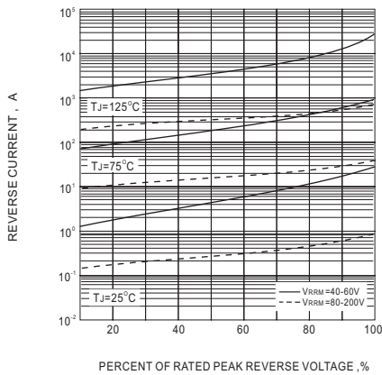
Fig. 3-TYPICAL REVERSE CHARACTERISTIC
