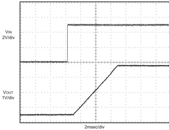
Start-Up from VIN (IOUT = 3.3V/10A, CIN/COUT = 22μF)
