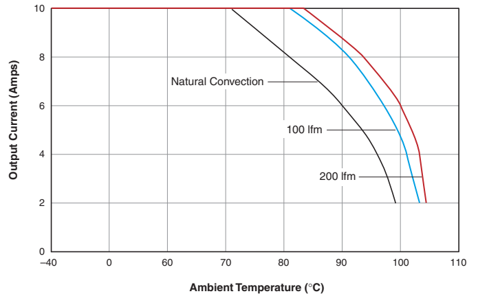
LSM-1/10-D5 Output Current vs. Ambient Temperature (SMT mount, air flow direction from pin 2 to pin 1)
