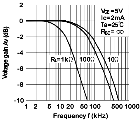
Fig.11 Frequency Response
