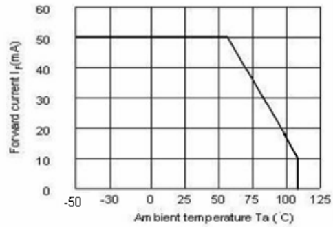
Fig.1 Forward Current vs. Ambient Temperature
