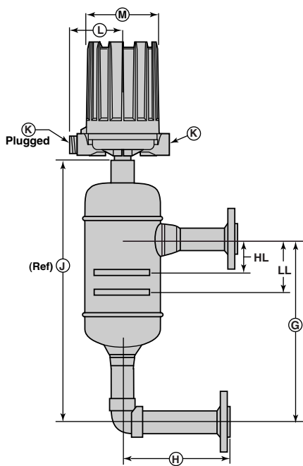
Figure 14 Flanged Side/Side
