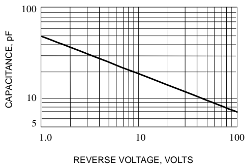
Fig. 5-TYPICAL JUNCTION CAPACITANCE PER BRIDGE ELEMENT
