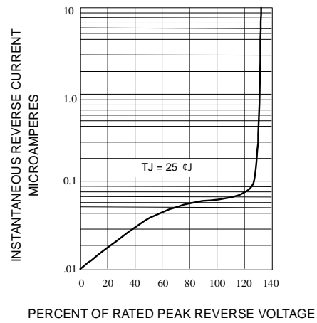
Fig. 4-TYPICAL REVERSE CHARACTERISTICS
