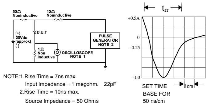
Fig. 6-REVERSE RECOVERY TIME CHARACTERISTIC AND TEST CIRCUIT DIAGRAM
