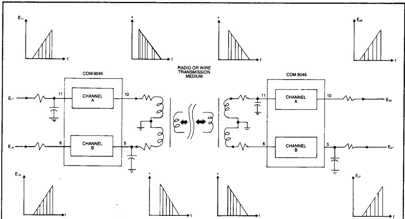
Figure 2 TYPICAL APPLICATION
