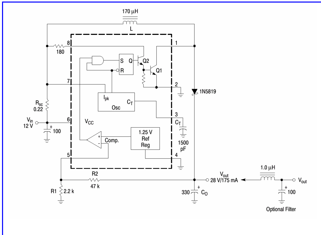
Figure 8. Step-Up Converter
