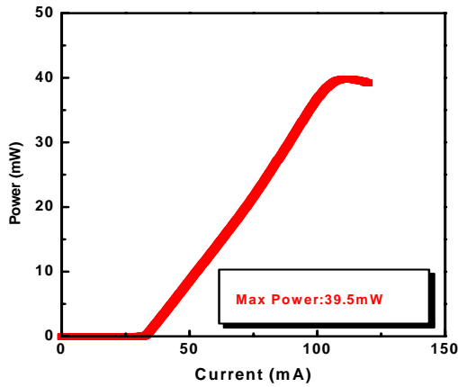
Max Power
