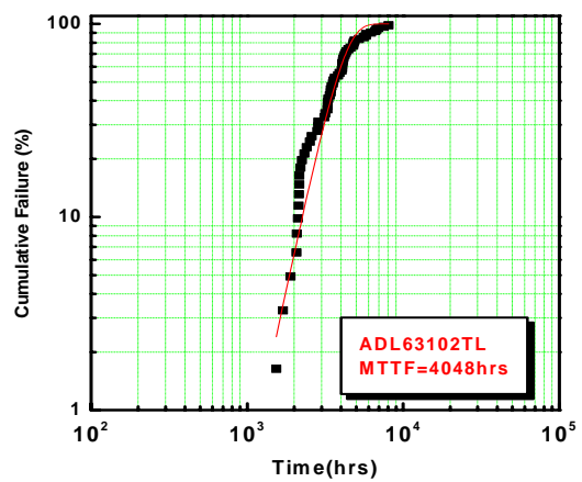
MTTF
