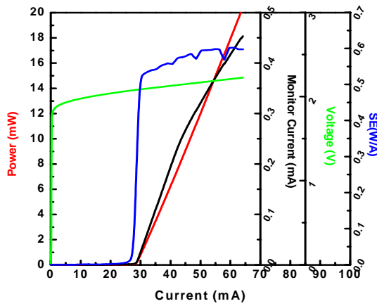
Laser characteristics
