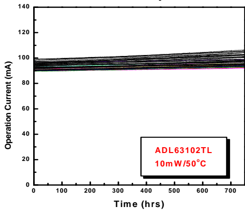
Reliability
