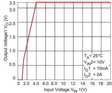
Figure 2. Output Voltage 1 vs. Input Voltage
