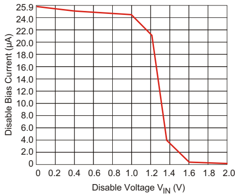
Figure 5. Disable Bias Current vs. Disable Voltage
