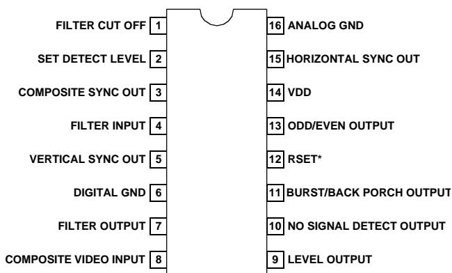
EL4583 (16-PIN SO, PDIP) TOP VIEW
