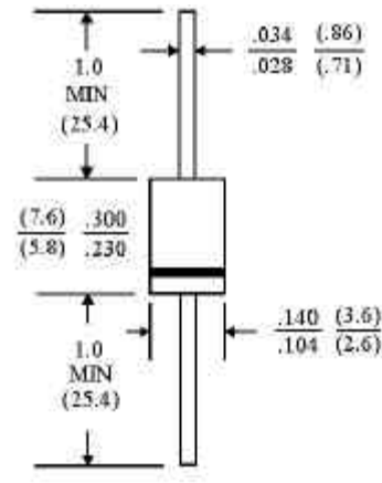
DO-15
