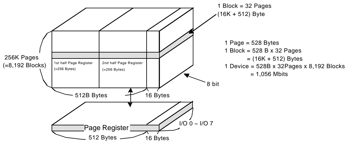
Figure 2. Array Organization
