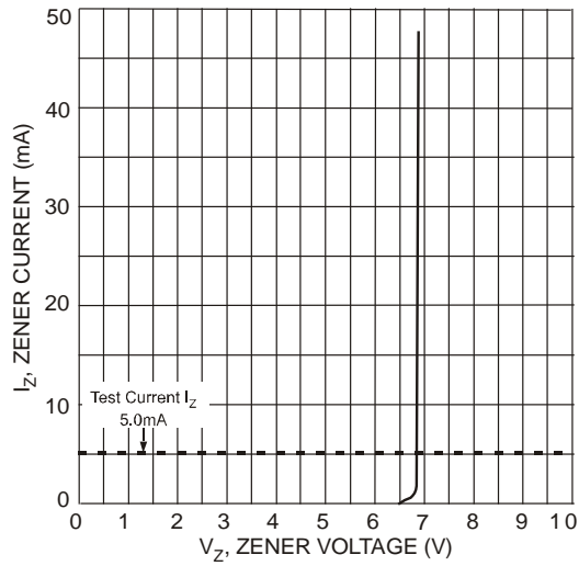
Fig. 1 Typical Zener Breakdown Characteristics
