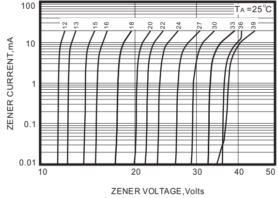
Fig.8 ZENER VOLTAGE VERSUS ZENER CURRENT
