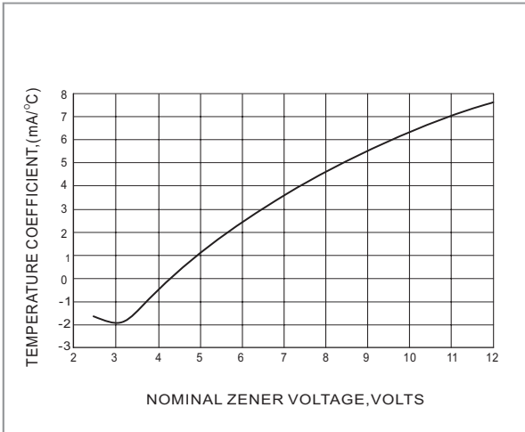
Fig.1 TEMPERATURE COEFFICIENTS
