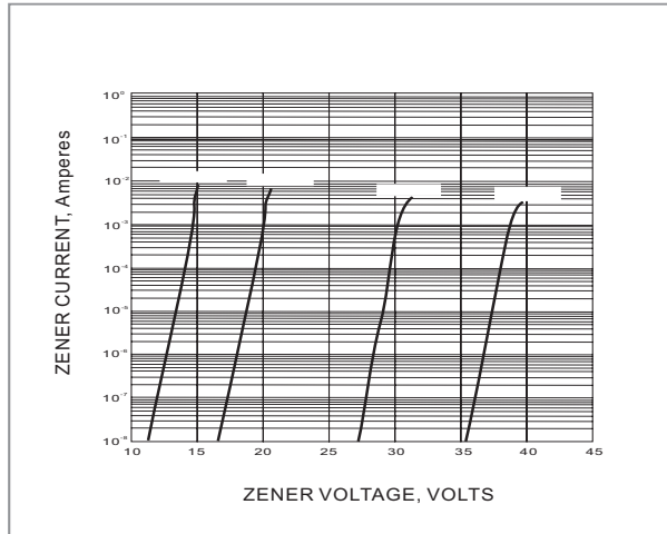
Fig.8 ZENER VOLTAGE VERSUS ZENER CURRENT
