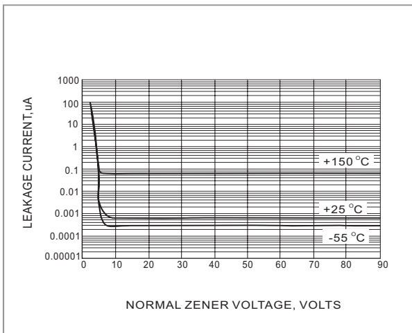
Fig.9 TYPICAL LEAKAGE CURRENT
