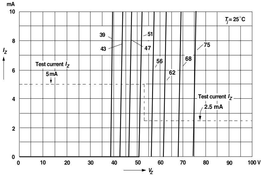
Figure 18. Breakdown Characteristics
