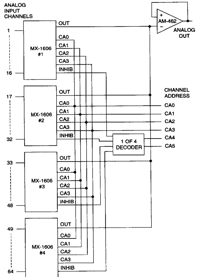
Figure 2. Expansion to 64 Channels
