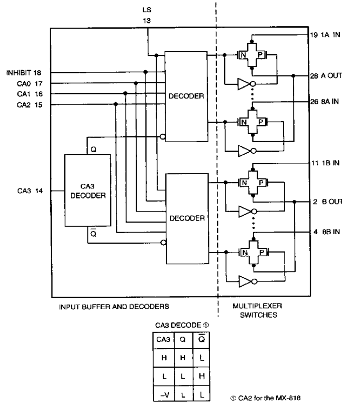
Figure 1. Functional Block Diagram (MX-1616 Pinout Shown)
