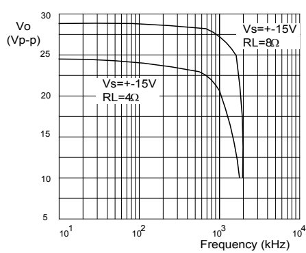
Fig.6 Large signal frequency response
