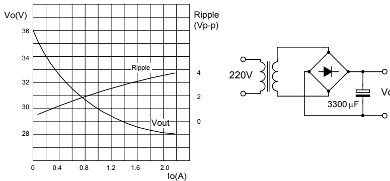
Fig.27 DC characteristics of 50W non-regulated supply
