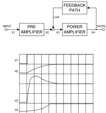
Fig.22 Overshoot phenomenon in feedback amplifiers
