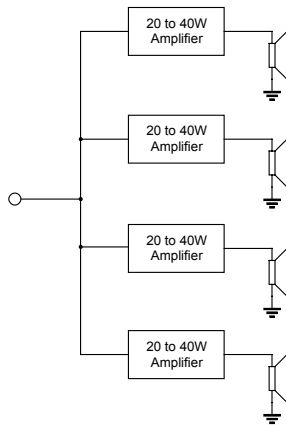
Fig.21 High power active box for musical instrument
