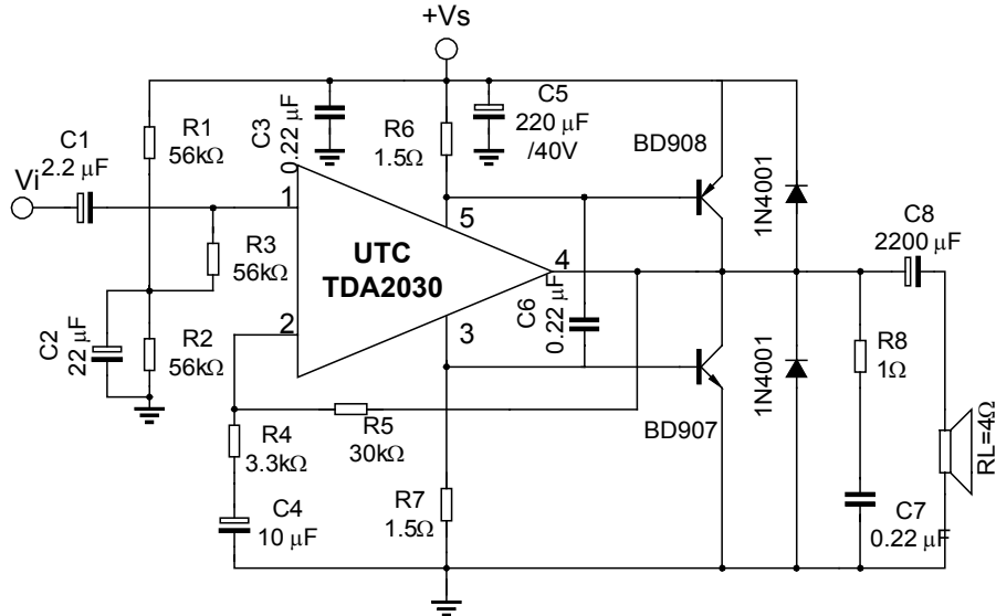
Fig. 8 Single supply high power amplifier(UTC TDA2030+BD908/BD907)
