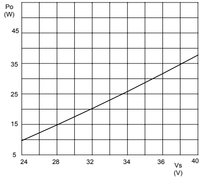
Fig. 10 Output power vs. supply voltage
