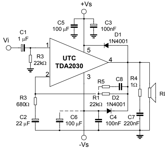
Fig. 14 Typical amplifier with split power supply
