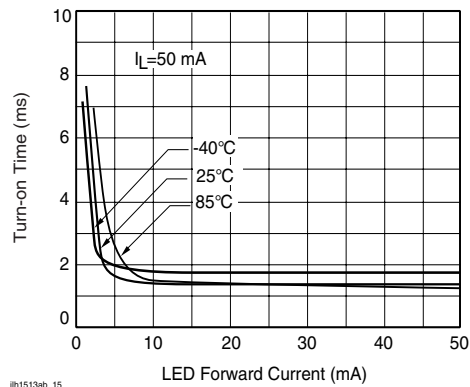
Figure 16. Turn-on Time vs. LED Current
