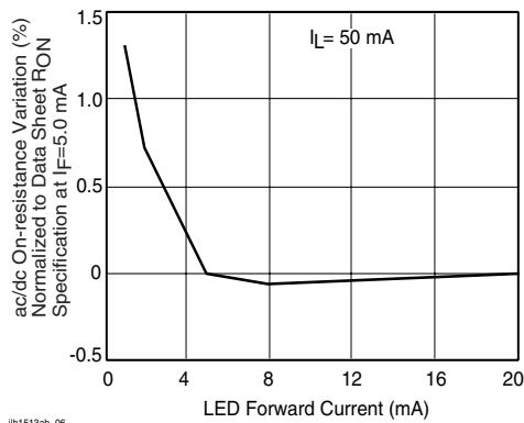
Figure 7. Variation in ON-Resistance vs. LED Current
