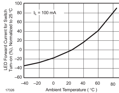
Figure 3. LED Current for Switch Turn-on vs. Temperature
