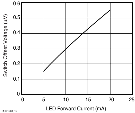
Figure 17. Switch Offset Voltage vs. LED Current
