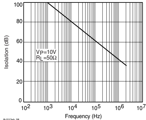
Figure 9. Output Isolation
