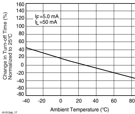
Figure 18. Turn-off Time vs. Temperature
