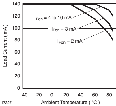
Figure 1. Recommended Operating Conditions
