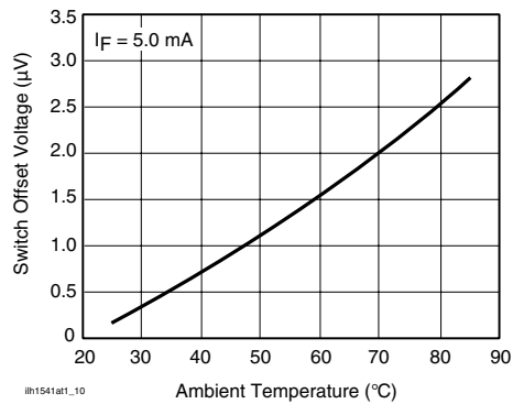
Figure 11. Switch Offset Voltage vs. Temperature
