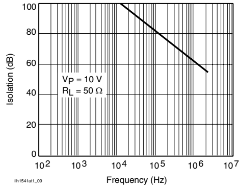
Figure 10. Output Isolation
