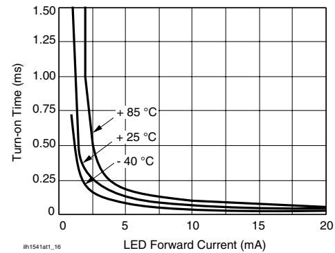
Figure 17. Turn-on Time vs. LED Current
