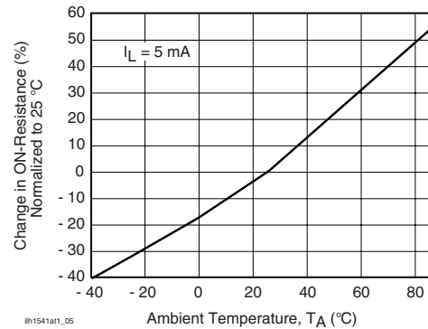
Figure 6. ON-Resistance vs. Temperature
