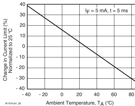
Figure 3. Current Limit vs. Temperature
