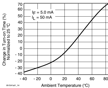
Figure 15. Turn-on Time vs. Temperature
