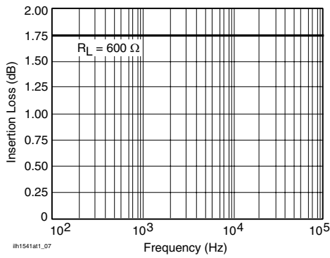
Figure 8. Insertion Loss vs. Frequency
