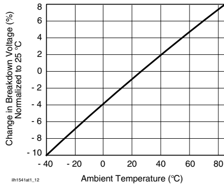
Figure 13. Switch Breakdown Voltage vs. Temperature
