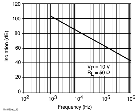
Figure 14. Output Isolation
