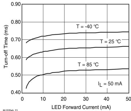
Figure 22. Turn-off Time vs. LED Current
