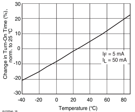
Figure 19. Turn-on Time vs. Temperature
