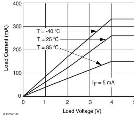
Figure 8. Load Current vs. Load Voltage
