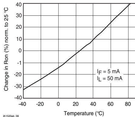
Figure 9. ON-Resistance vs. Temperature
