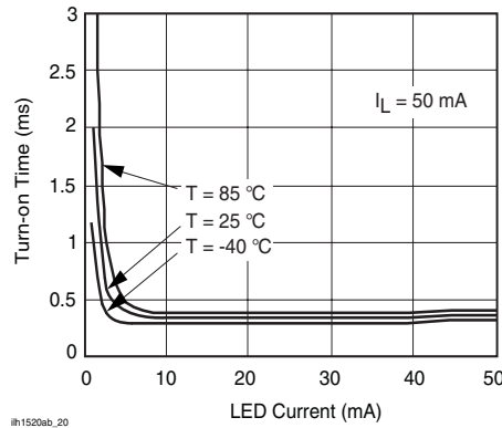
Figure 21. Turn-on Time vs. LED Current
