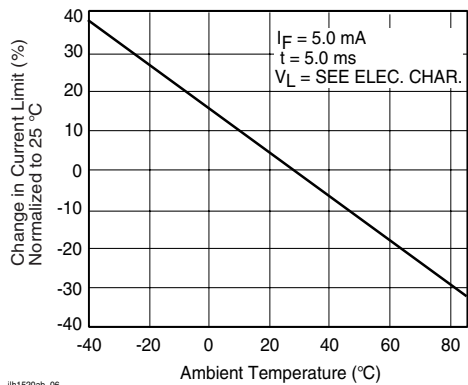
Figure 7. Current Limit vs. Temperature
