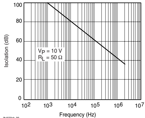
Figure 10. Output Isolation
