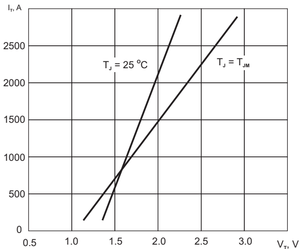
Limiting on-state characteristic I_T = f(V_T)
