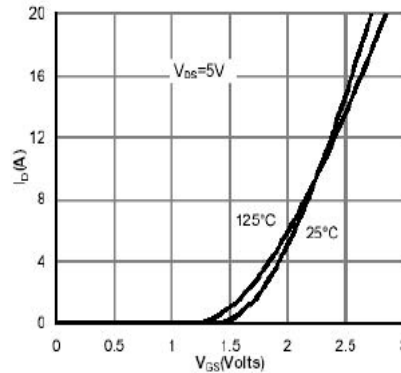
Figure 2: Transfer Characteristics
