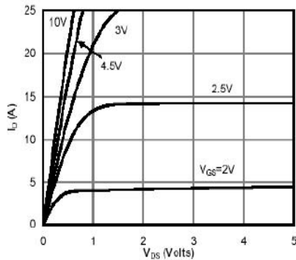
Fig 1: On-Region Characteristics
