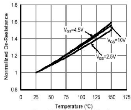
Figure 4: On-Resistance vs. Junction Temperature
