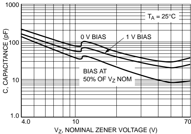
Figure 3. Typical Capacitance
