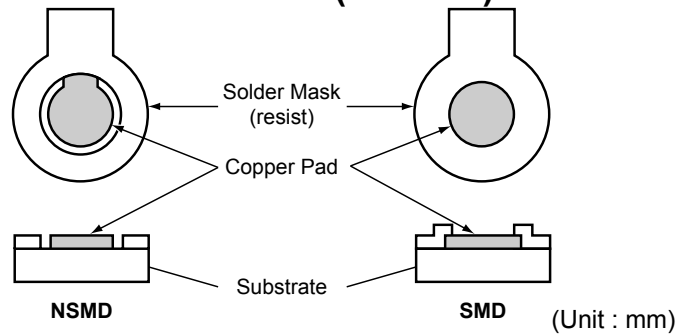
NSMD and SMD Pad Definition
