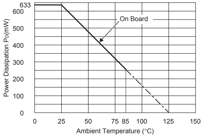
Power Dissipation
