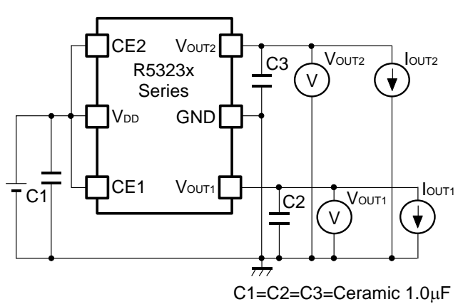
Fig.1 Standard test Circuit
