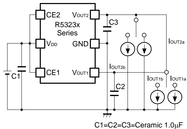
Fig.4 Load Transient Response Test Circuit
