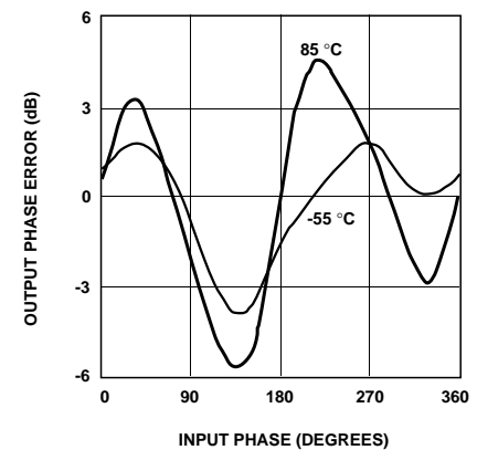
Figure 50. HPMX-2003 Vector Phase Error vs. Input Phase and Temperature at 950\text{ MHz} , V_{CC} = 5\text{ V} , LO = -12\text{ dBm} , Unbalanced, V_{\text{Iref}} = V_{\text{Qref}} = 2.5\text{ V} .
