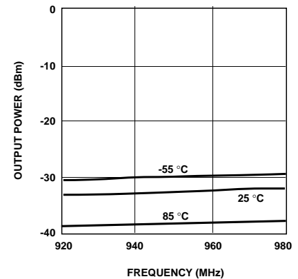
Figure 47. LO Leakage vs. Frequency and Temperature (With 25^{\circ}\text{C} Offset Adjustment), V_{CC} = 5\text{ V} , LO = -12\text{ dBm} , V_{\text{Iref}} = V_{\text{Qref}} = 2.5\text{ V} .
