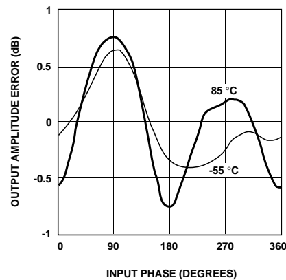
Figure 49. HPMX-2003 Vector Amplitude Error vs. Input Phase and Temperature at 950\text{ MHz} , V_{CC} = 5\text{ V} , LO = -12\text{ dBm} , Unbalanced, V_{\text{Iref}} = V_{\text{Qref}} = 2.5\text{ V} .
