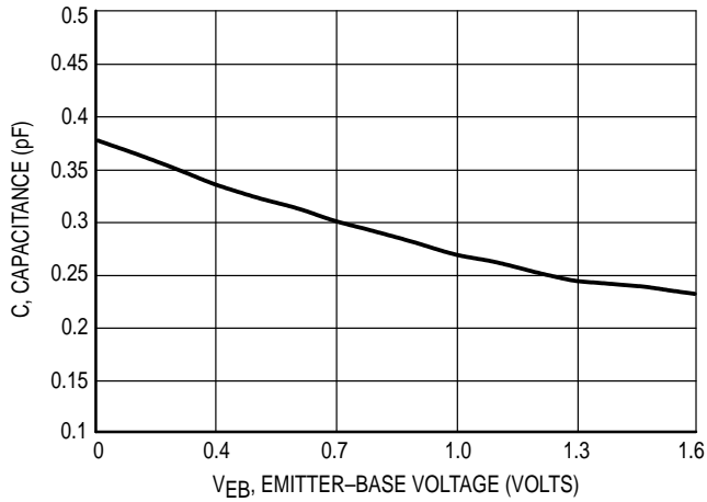
Figure 1. C_{je} Input Capacitance versus Voltage
