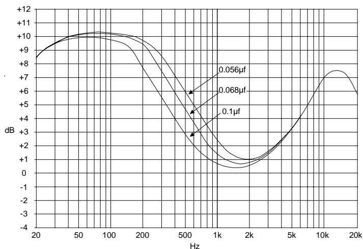
BL1—BL2 Capacitor vs. Frequency Response Curve
