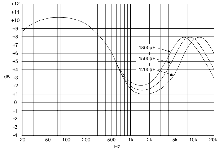
TL-OUTL Capacitors vs. Frequency Response
