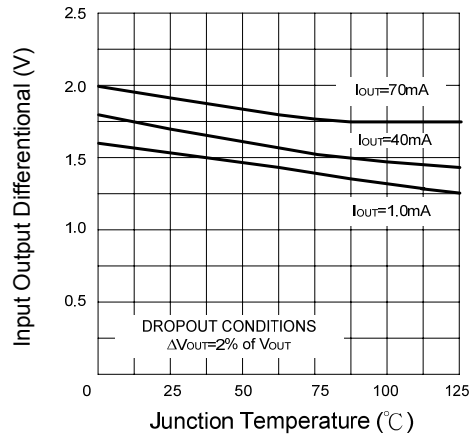
Fig.10 Dropout Voltage
