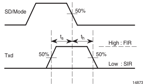
Figure 2. Mode Switching Timing Diagram
