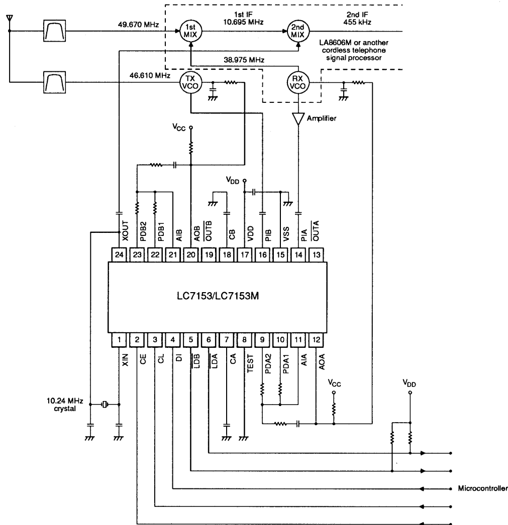
Figure 5. American 10-channel, 46/49 MHz, cordless telephone base station
