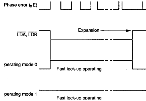
Figure 4. Fast lock-up operating modes
