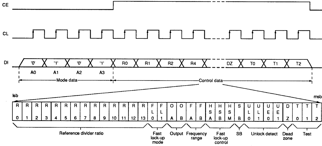
Figure 3. Mode 2 command (reference divider and control data)
