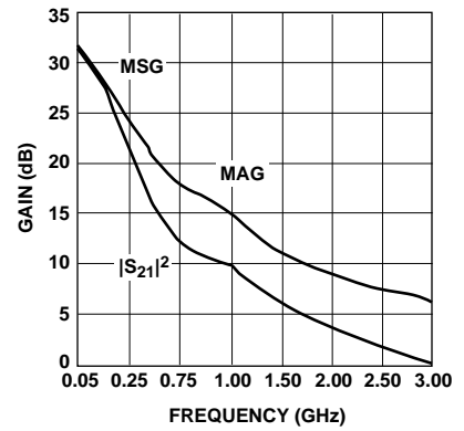
Figure 16. Insertion Power Gain, Maximum Available Gain, and Maximum Stable Gain vs. Frequency. V_{CE} = 6.0V , I_C = 50 \text{ mA} .
