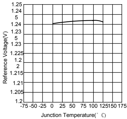
Figure 3. Reference Voltage vs. Temperature
