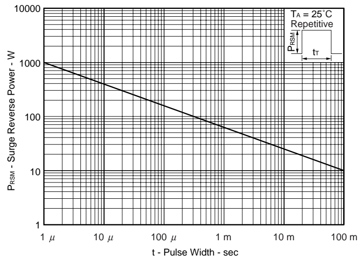
Fig.6 SURGE REVERSE POWER RATINGS
