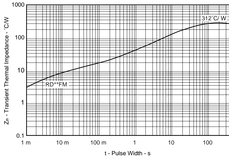
Fig.5 TRANSIENT THERMAL IMPEDANCE CHARACTERISTICS
