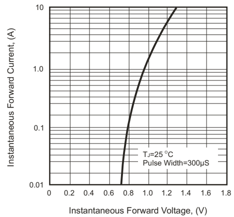
Fig.4-Typical Forward Characteristics
