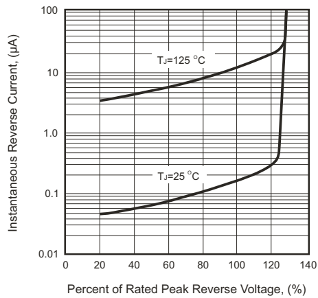
Fig.3-Typical Reverse Characteristics
