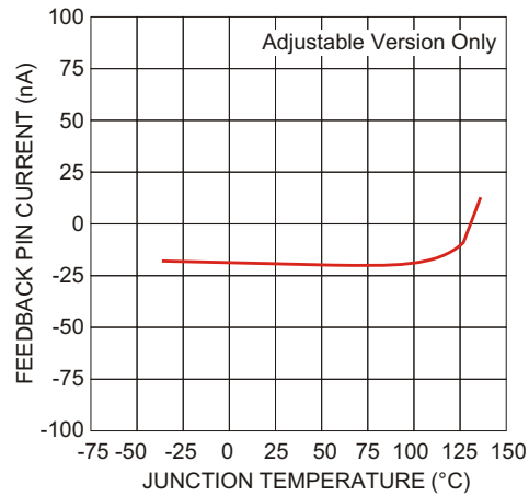
Figure 11. Feedback Pin Current
