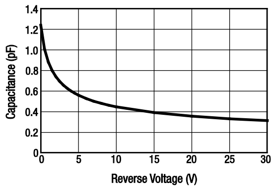
Figure 3. Capacitance vs Reverse Voltage (SMV1430)
