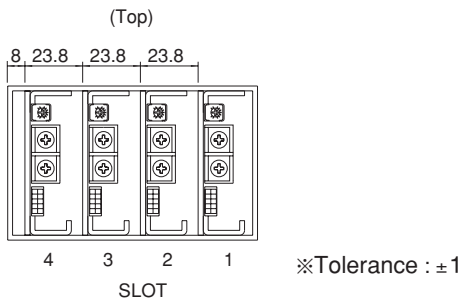
ACE300F Output side view
