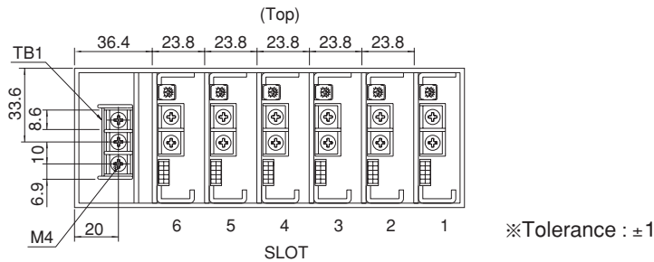
ACE900F Output side view
