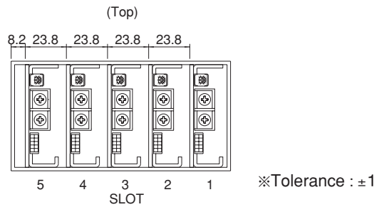
ACE450F/650F Output side view
