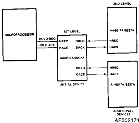
Figure 1. Cascaded Am9517A/8237As
