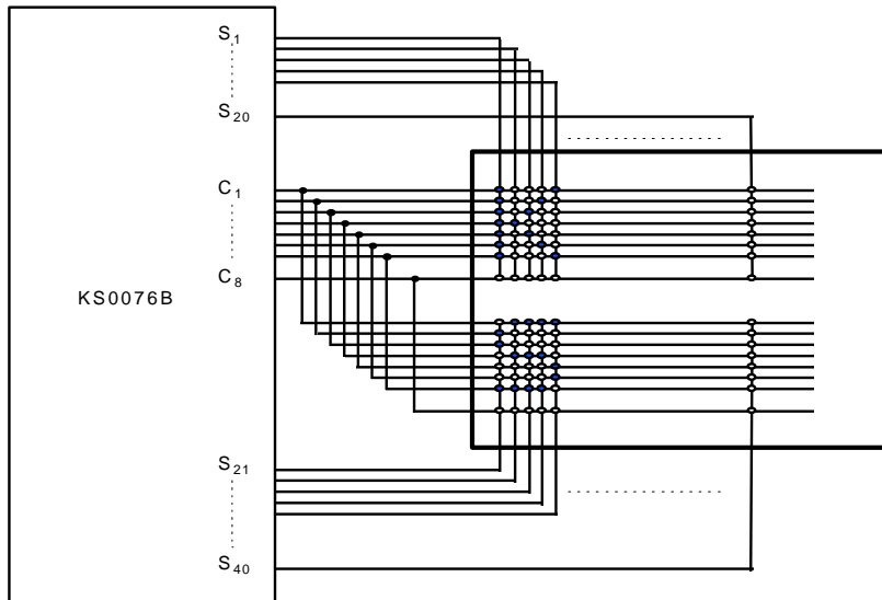
DIVIDE CIRCUIT
