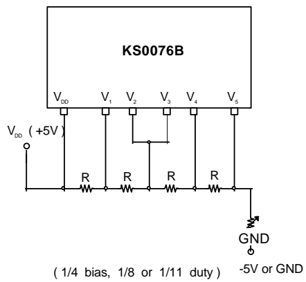
DIVIDE CIRCUIT
