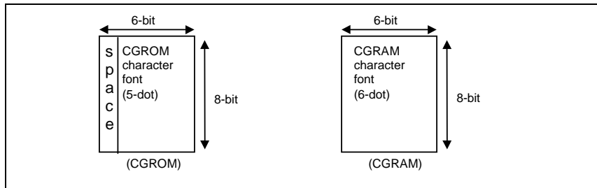
Fig-9. 6-dot font width CGROM/CGRAM
