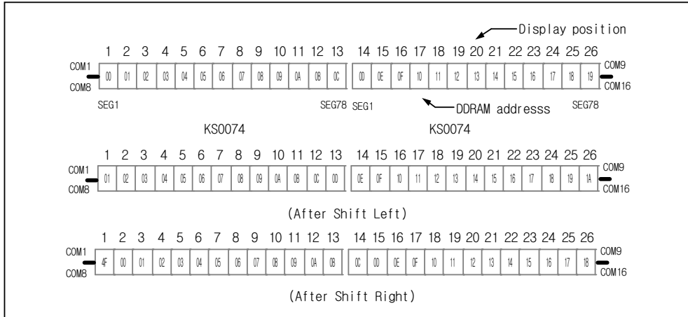
Fig-5. 1-line X 26ch. display
