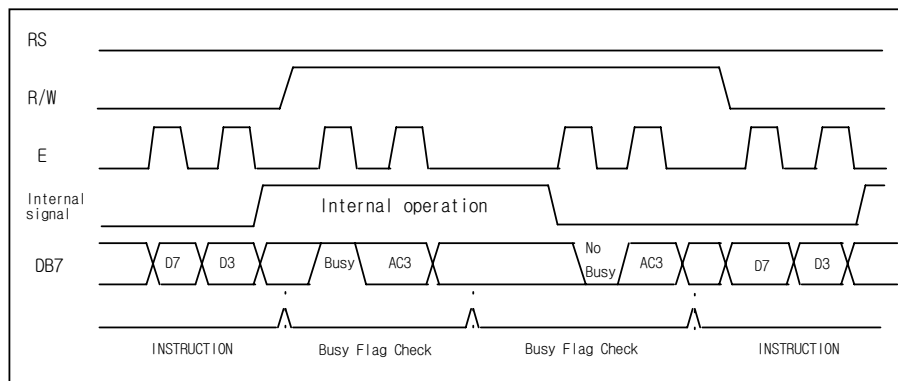
Fig 12. Example of 4-bit Bus Mode Timing Sequence
