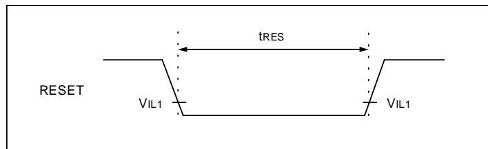
Fig-18. Reset Timing Diagram
