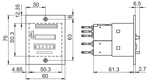
FE514 front panel with 2 screws
