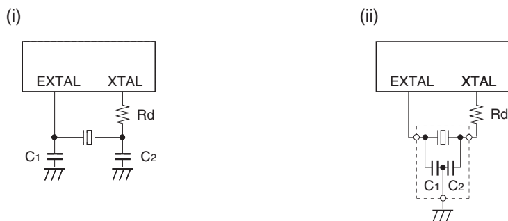
Fig. 13. SPC700 Series recommended oscillation circuit
