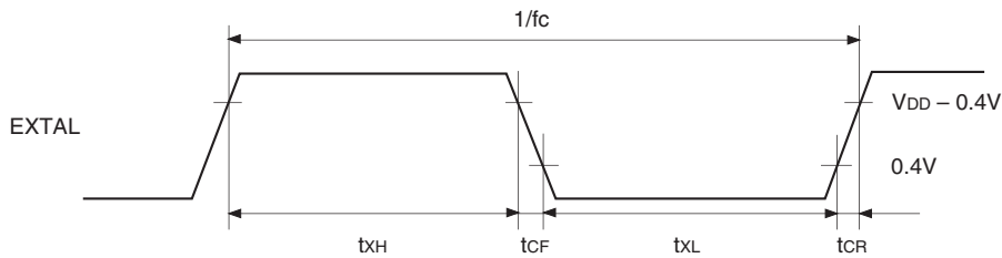
Fig. 2. Clock applied condition
