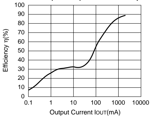
R1224N502H (V IN =15V) CDRH127-10μH
