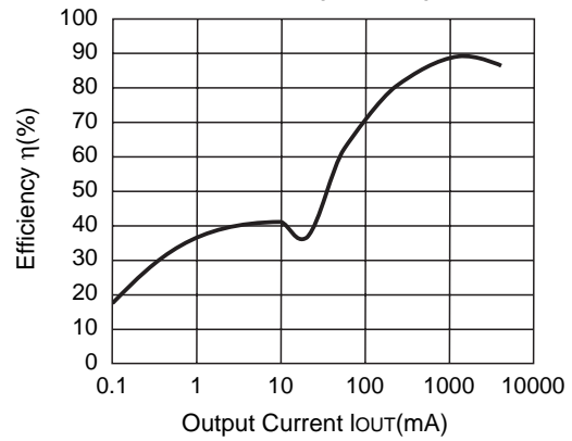
R1224N332G (V IN =10V)
