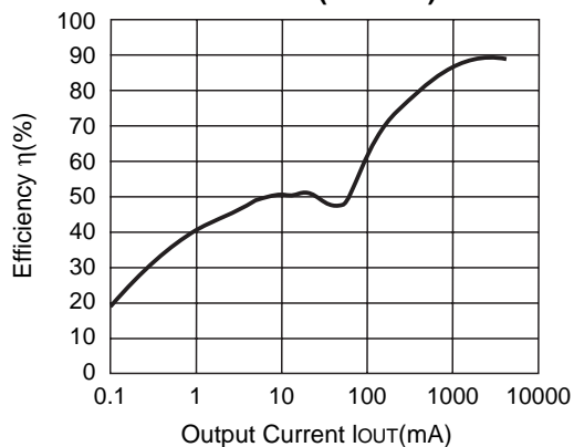
R1224N502G ( V_{IN}=16V )
