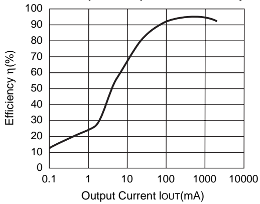
R1224N332M (V IN =4.8V) CDRH127-27μH
