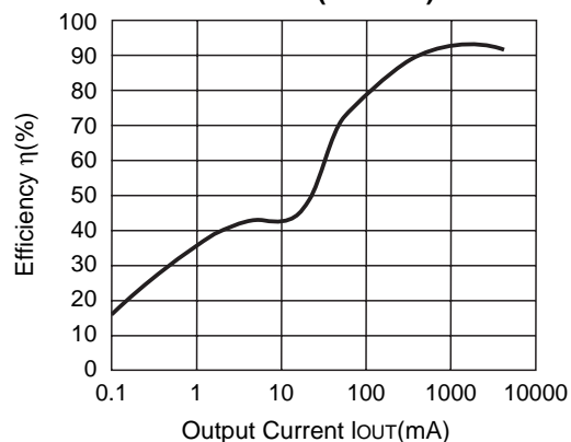
R1224N502G ( V_{IN}=10V )
