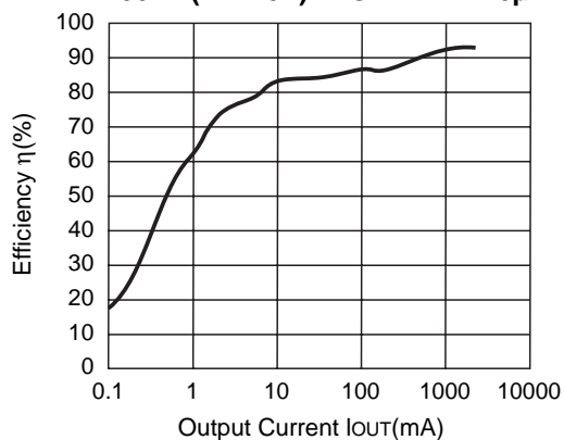
R1224N502E ( V_{IN}=10V ) CDRH127-10 \mu H
