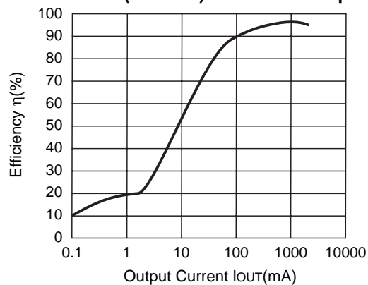
R1224N502G ( V_{IN}=6.5V ) CDRH127-10 \mu H
