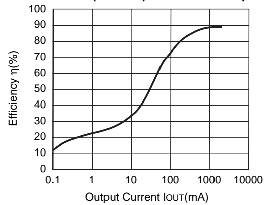
R1224N332M (V IN =12V) CDRH127-27μH
