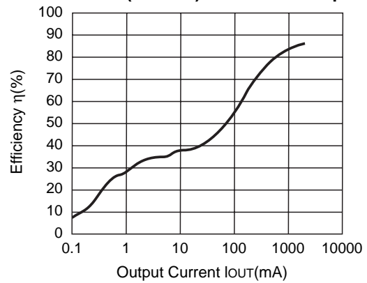
R1224N332G (V IN =15V) CDRH127-10μH
