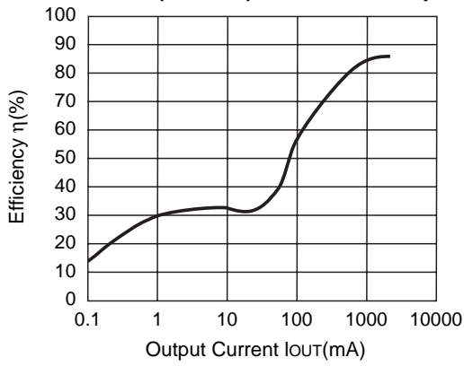
R1224N332H (V IN =12V) CDRH127-10μH
