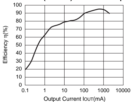
R1224N332E ( V_{IN}=4.8V ) CDRH127-10 \mu H
