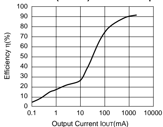
R1224N502M ( V_{IN}=15V ) CDRH127-27 \mu H
