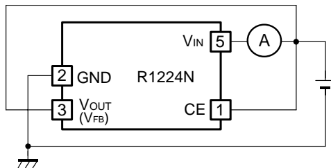
Supply Current 1
