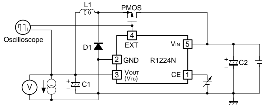
Supply Current 1
