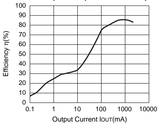
R1224N182H (V IN =5.0V) CDRH127-10μH
