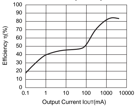
R1224N332G (V IN =16V)
