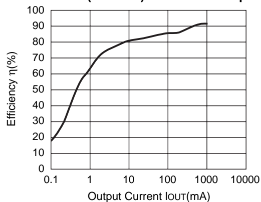
R1224N332E ( V_{IN}=7.0V ) CDRH127-10 \mu H
