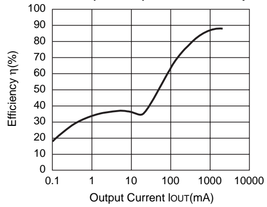
R1224N332G (V IN =12V) CDRH127-10μH
