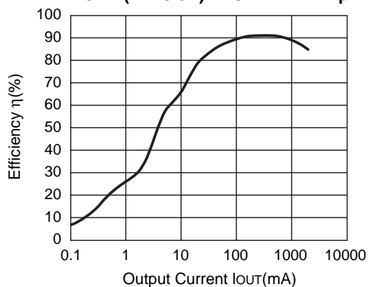
R1224N182M ( V_{IN}=3.3V ) CDRH127-27 \mu H
