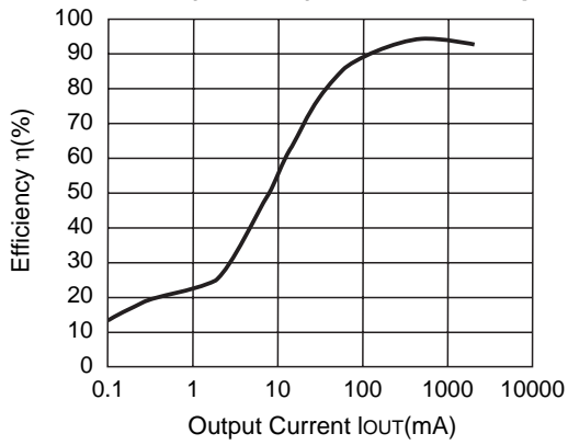
R1224N332G (V IN =4.8V) CDRH127-10μH
