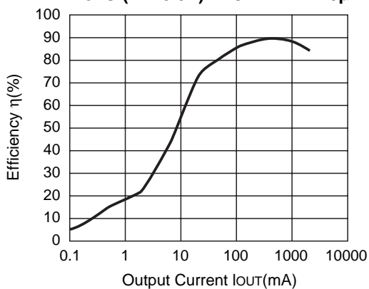
R1224N182G (V IN =3.3V) CDRH127-10 \mu H
