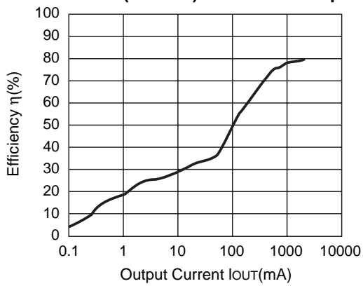
R1224N182G (V IN =12V) CDRH127-10μH
