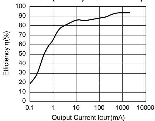
R1224N502L ( V_{IN}=10V ) CDRH127-27 \mu H
