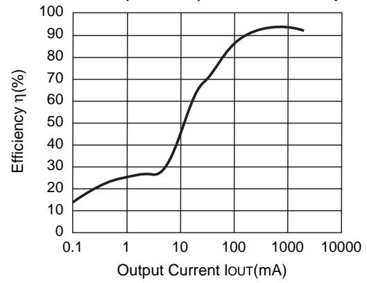
R1224N332H (V IN =4.8V) CDRH127-10μH
