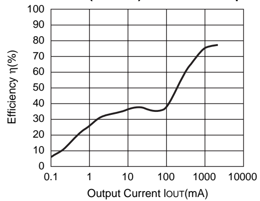
R1224N182H (V IN =12V) CDRH127-10μH
