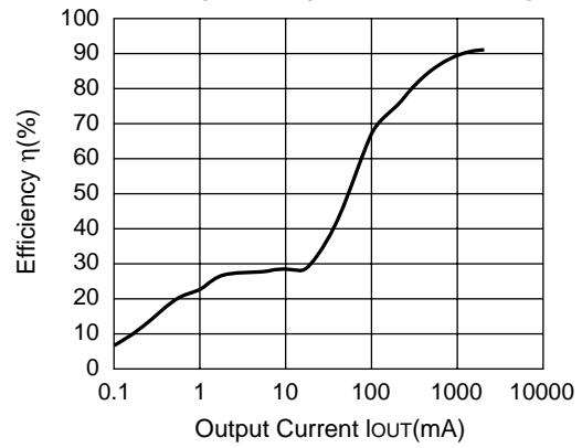
R1224N502H (V IN =12V) CDRH127-10μH
