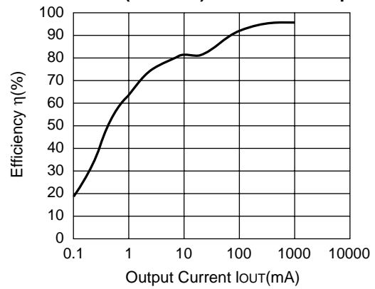
R1224N502L (V IN =6.5V) CDRH127-27μH
