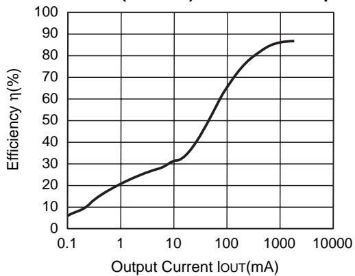
R1224N332M (V IN =15V) CDRH127-27μH
