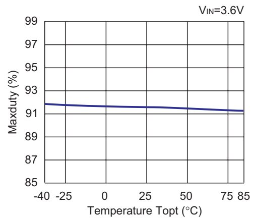
11) Maximum duty cycle vs. Temperature R1218x041A
