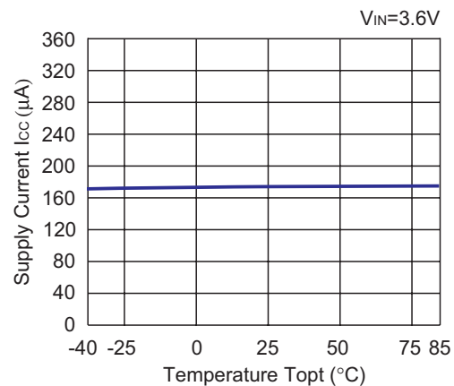
13) Supply Current vs. Temperature R1218x041A
