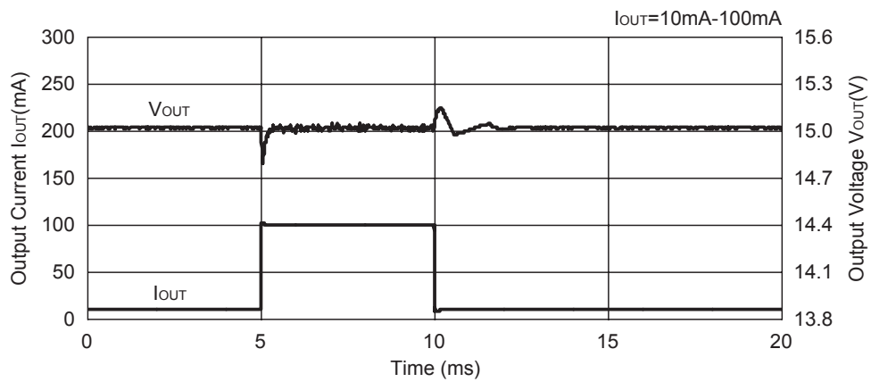
R1212D100B
