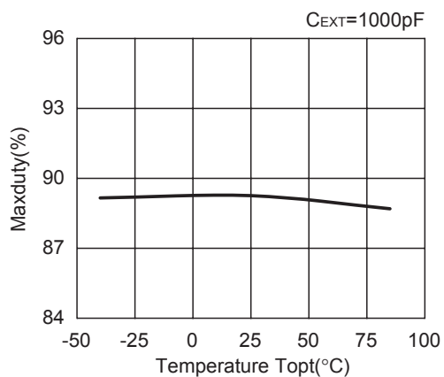
R1212D101A
