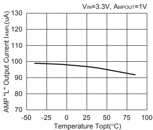
R1212D10xC
