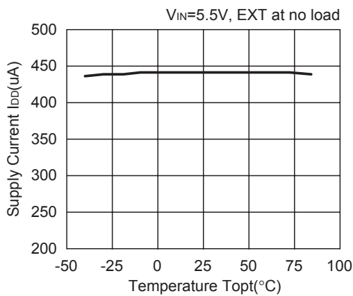
R1212D10xA
