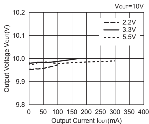
R1212D100B
