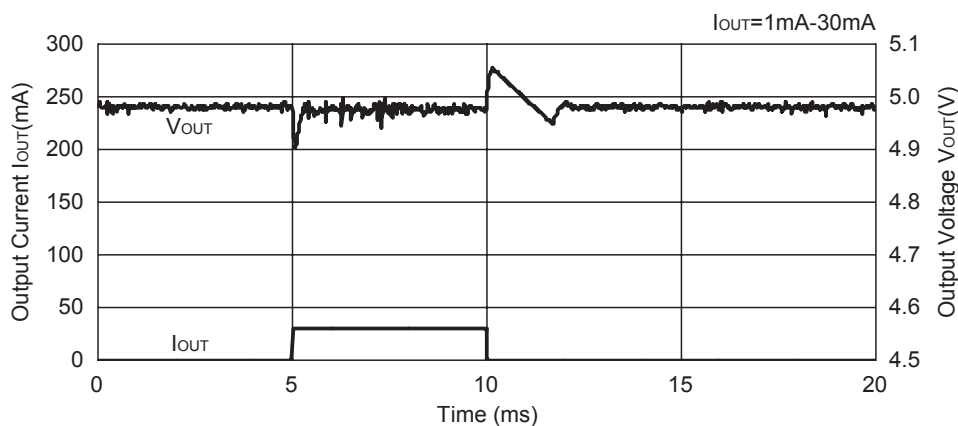
R1212D100B
