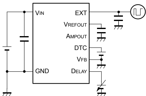
Fig.7 DELAY Pin Detector Threshold Test Circuit
