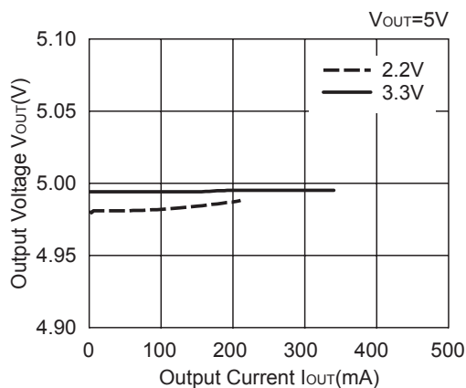
R1212D100A
