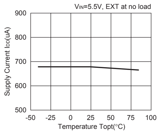
R1212D10xB
