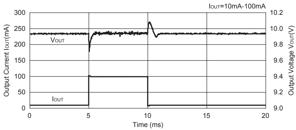
R1212D100B
