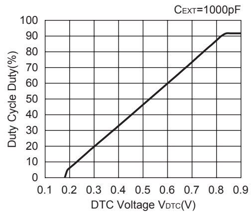
R1212D101C
