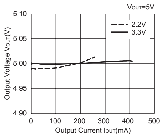
R1212D100B
