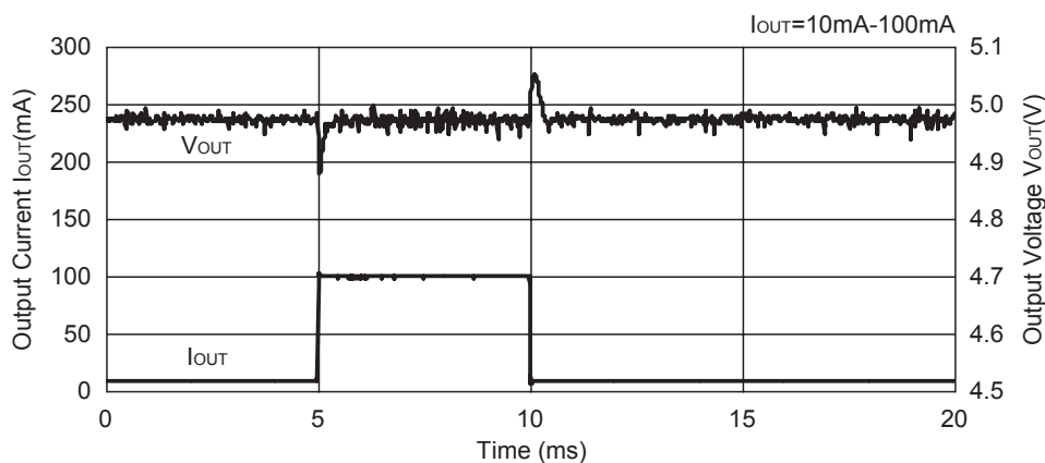
R1212D100B
