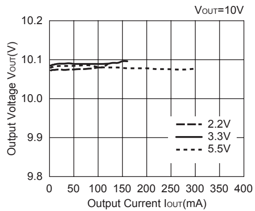
R1212D101C
