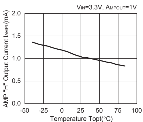
R1212D10xx
