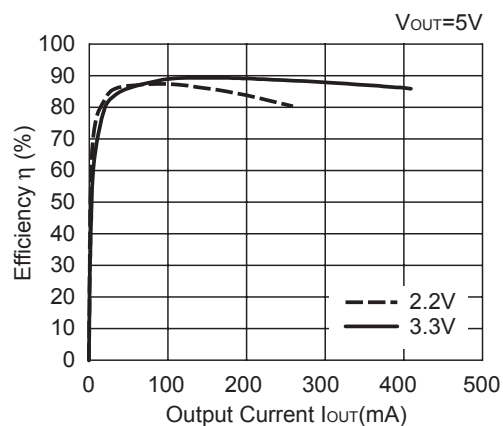
R1212D100B
