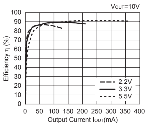
R1212D100B
