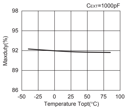
R1212D101C
