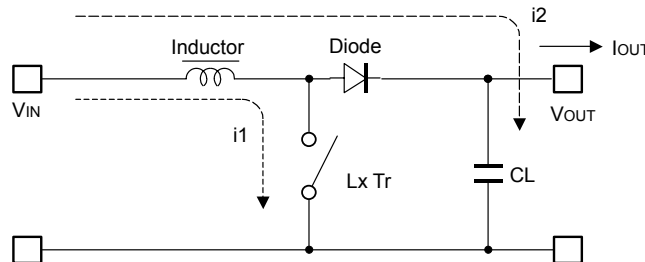
<Circuit through L>
