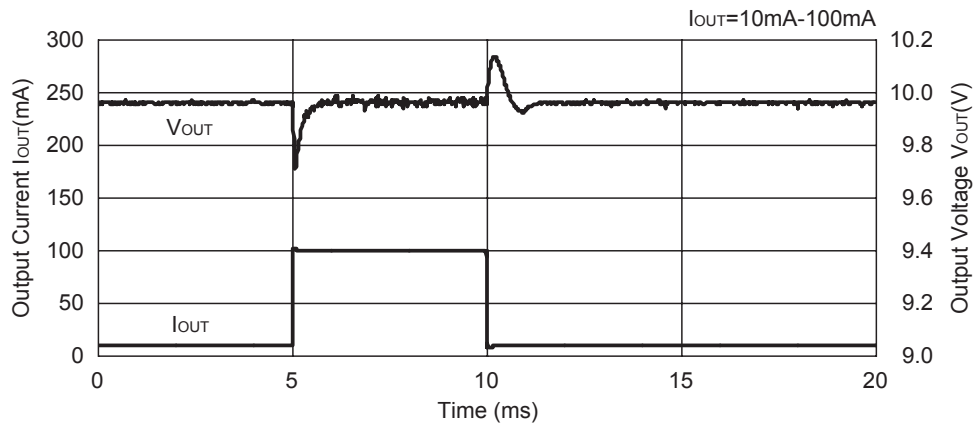
R1212D100A
