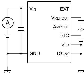
Fig.1 Consumption Current Test Circuit
