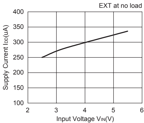
R1212D101C
